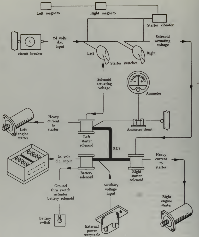
FIGURE 5-5. Engine starting schematic for a light twin-engine aircraft.
